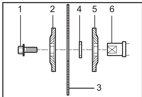
► 1. Hex socket bolt 2. Outer flange 3. Saw blade 4. Ring 5. Inner flange 6. Spindle
